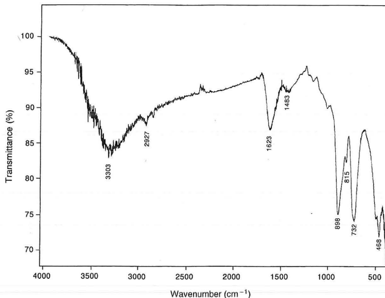
FIG. 3. Fourier-transform infrared spectrum of piritite from 400 to 4000 \text{cm}^{-1} .
